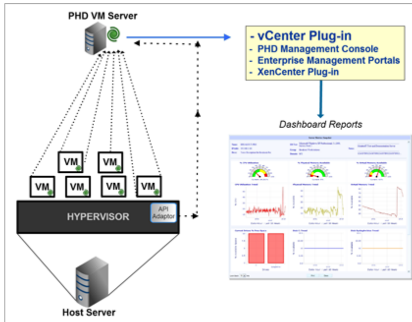
Figure 2 - Monitoring VMware vSphere Virtual Environment
